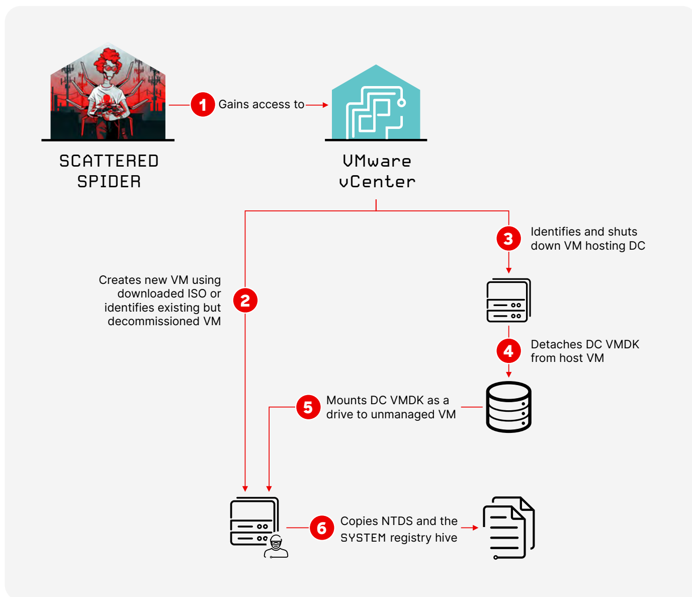
Figure 10. SCATTERED SPIDER leverages unmanaged VMs to dump credentials
