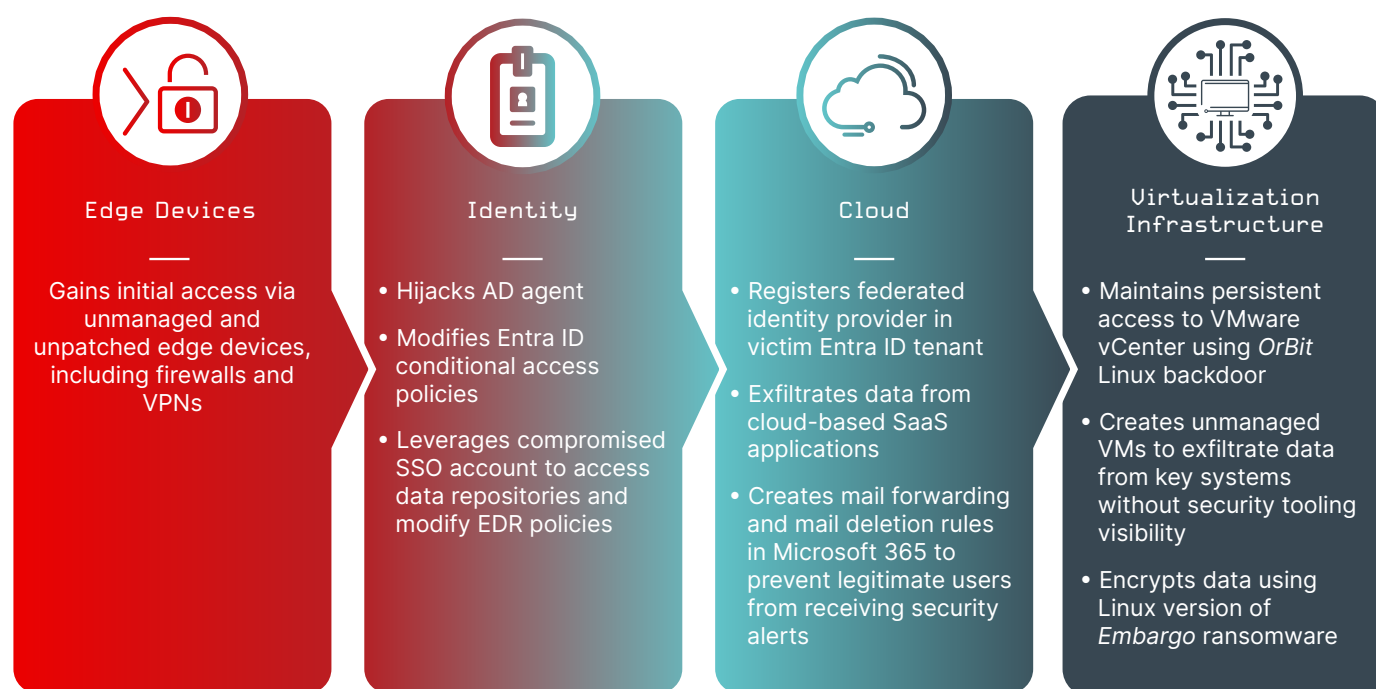
Figure 13. BLOCKADE SPIDER's cross-domain tradecraft
