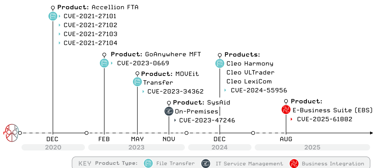
Figure 17. Zero-day vulnerabilities exploited by GRACEFUL SPIDER
