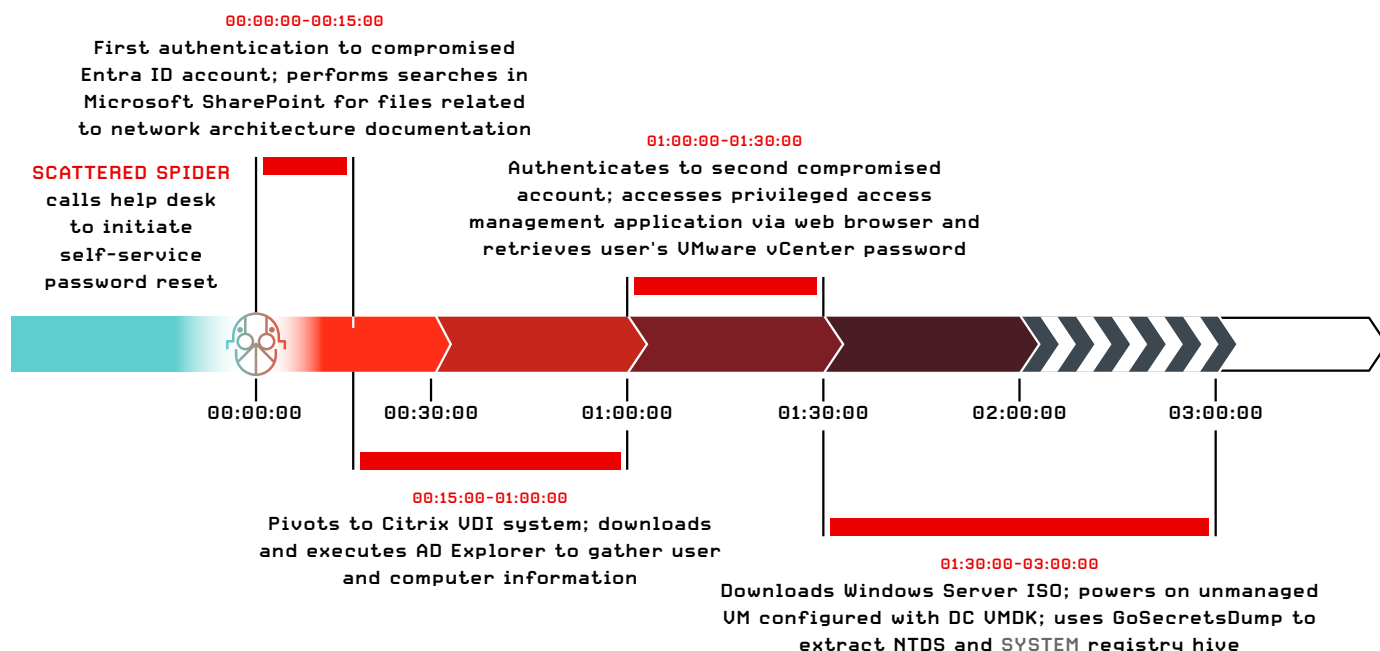
Figure 11. SCATTERED SPIDER dumps NTDS via unmanaged VM in three hours
