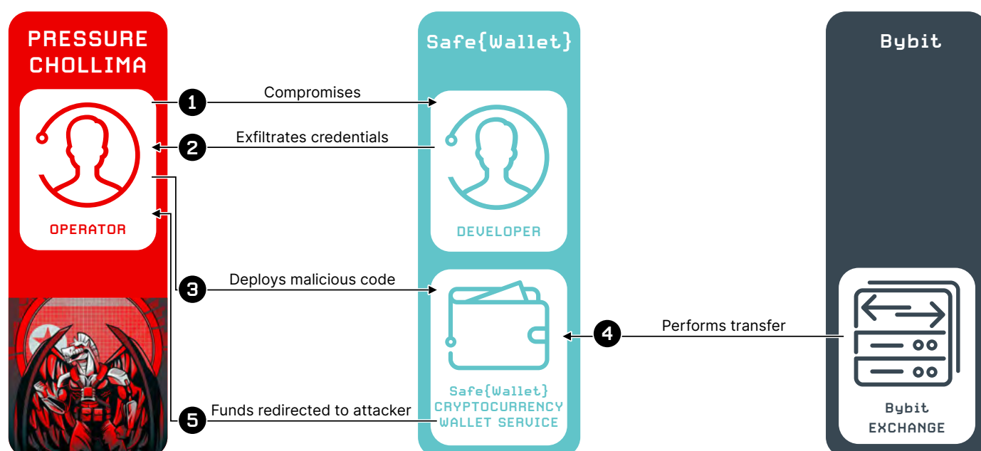
Figure 16. PRESSURE CHOLLIMA supply chain attack targeting Bybit
